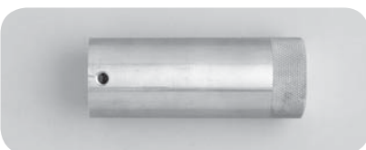
436272 Twin Cutter Extension Knob Extends right hand twin cutter adjustment knob for easier adjusting.
