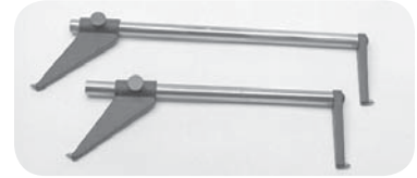
FOR DRUMS Drum Wear Limit Gauges Designed to determine whether worn or scored brake drums can be safely machined. 434287 Drum Wear Limit Gauge, Passenger Car, 8"-14" (204-355 mm). 436367 Drum Wear Limit Gauge, Passenger Cars Through Trucks, 6"-22" (150-560 mm).
